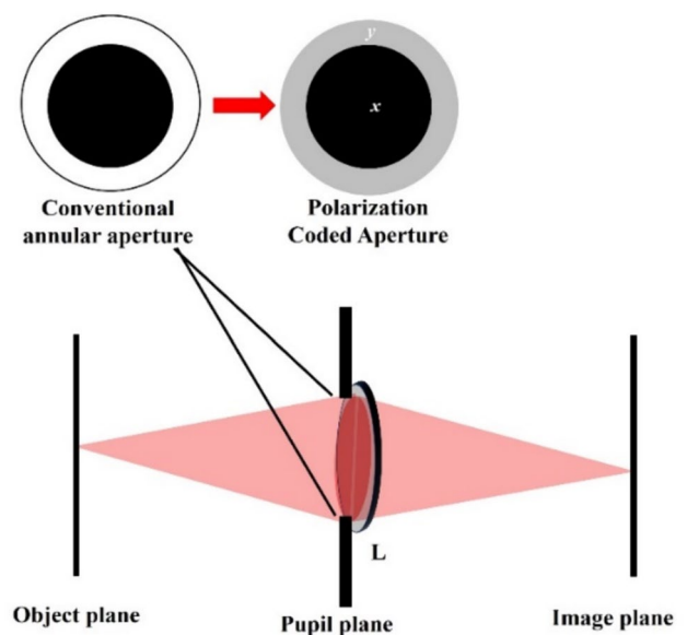
Fig. 57 Schematic of PCA equipped imaging of diffraction-limited imaging lens. Inset shows a design of Polarization encrypted annular (ring) aperture by the OPM method
