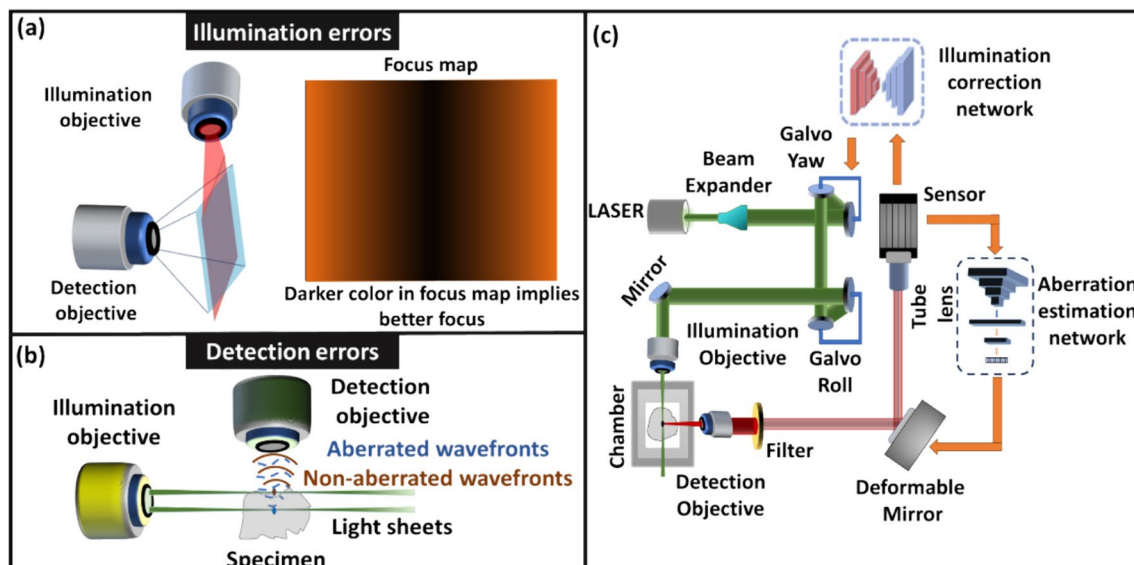
Fig. 10 a Illumination and b detection errors in LSFM. c Experimental schematic for correcting the illumination and detection errors in a custom-LSFM, with a deformable mirror, and two galvo mirrors
