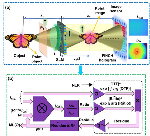
Fig. 6 a Optical configuration of FINCH as CAI. b Schematic of LRRA
