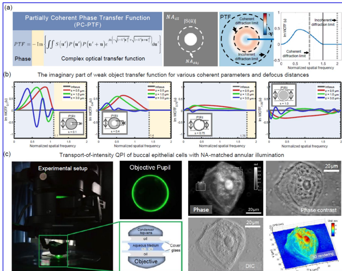
Fig. 27 QPI under partially coherent illumination. a Partially coherent phase transfer function. b The imaginary part of weak object transfer function for various coherent parameters and defocus distances.
