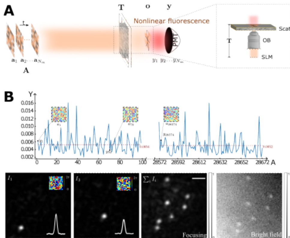
Fig. 44 A single-pixel approach to recover the transmission matrix. A Simplified schematic view of a general fluorescence microscope with a single-pixel detector. Random wavefront generated by a SLM a_{N_m} impinges on a scattering medium with a transmission matrix T and excites 2-photon fluorescence (2PF) of an extended object o . The fluorescence signal y is collected by a single-pixel detector (e.g. photomultiplier tube (PMT)). A matrix A is made from the known wavefronts a_{N_m} . A gradient-descent-based algorithm is used to solve the forward problem \min_{\mathbf{t}_i} \|\mathbf{y} - \sum |\mathbf{A}\mathbf{t}_i|^4\|^2 , where \mathbf{t}_i are filtered columns of
