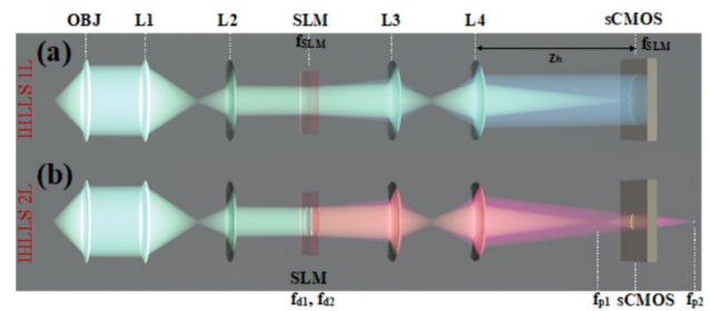
Fig. 13 Optical configuration of IHLLS [97]; f_{\text{SLM}} = 400 mm, f_{d1} = 435 mm, f_{d2} = 550 mm; here, we chose two focal lengths of size closer to the calibration focal length
