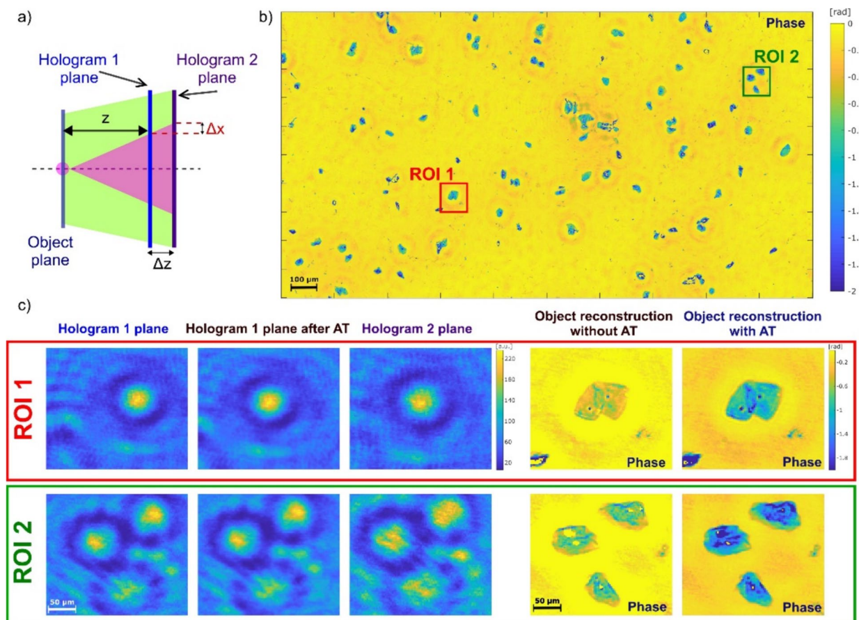
Fig. 34 Twin-image removal in the in-line lensless digital holography microscopy by multi-height hologram acquisition. a The idea of the method. \Delta z denotes the hologram (sensor) axial (longitudinal) plane shift and \Delta x denotes the in-plane (transversal) shift of the hologram features positions for the two hologram planes. b The phase image of
