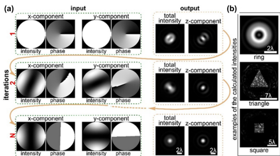
Fig. 52 Calculation results: a Iterative procedure of the design of an element concentrating energy in a circle with radius 0.5 \lambda , b examples of the total intensity distributions shaped with designed elements
