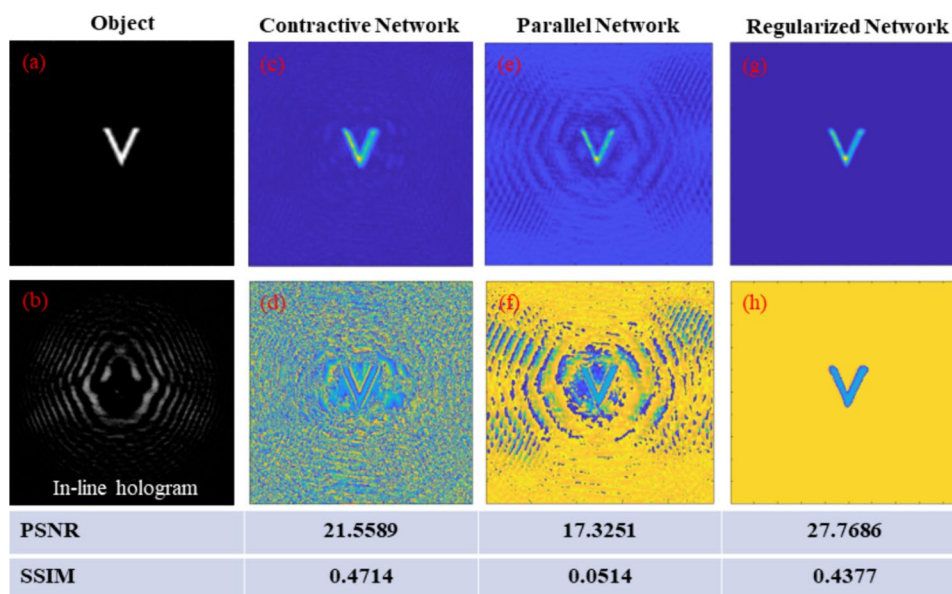
Fig. 43 Experimental results: a object “V” displayed using SLM, b intensity distribution of recorded in-line hologram, c–h amplitude phase reconstruction results with various network architectures. The PSNR and SSIM comparison of various network architectures are given in the last two rows
