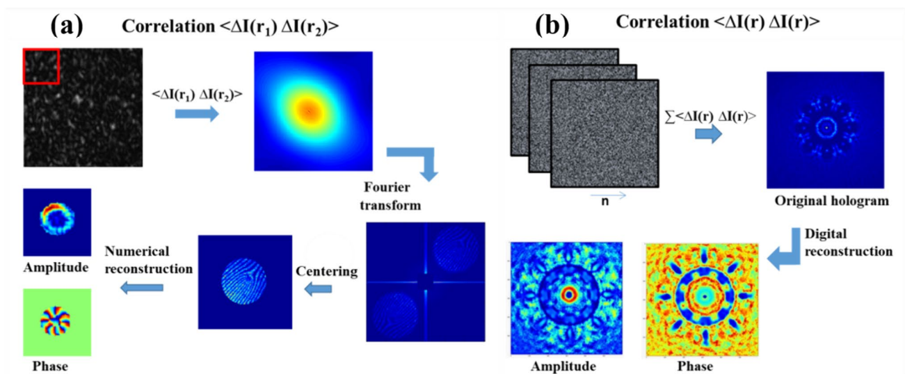
Fig. 51 A flow chart highlighting imaging of the complex valued object from post-processing of the random intensities a cross-correlation of intensities using spatial averaging, b auto-correlation of intensities and temporal averaging
