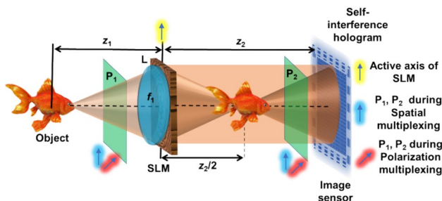
Fig. 4 Optical configuration of FINCH
