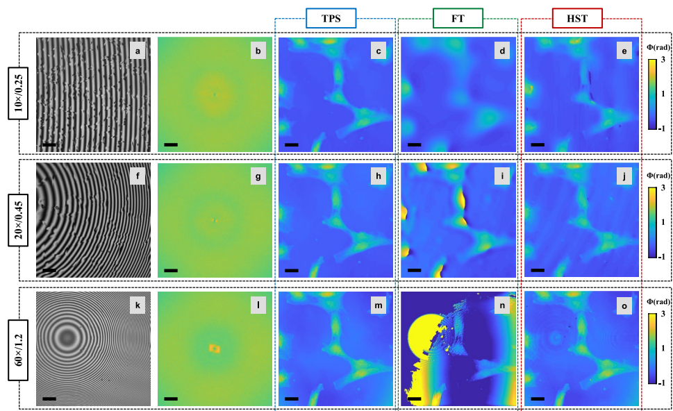
Fig. 37 Experimental results of MEF cells for 10 \times /0.25, 20 \times /0.45 and 60 \times /1.2 objective lenses: raw interferograms (a, f, k), FT spectra (b, g, l), phase reconstructed with TPS (c, h, m), phase reconstructed with FT (d, i, n) and phase reconstructed with HST (e, j, o). The imaging objective lens MO 2 as shown in Fig. 35 is changed while MO 1 was kept constant 10 \times /0.25 N.A
