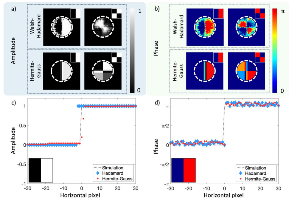
Fig. 18 a Amplitude and b phase reconstructions for a checkerboard pattern and a step object (shown as insets), using Hermite-Gauss (HG) and Walsh-Hadamard masks. The outer area of the dashed white circle represents the region where noise was suppressed due to lack of SPDC signal. 2D cross-sectional plots of the c amplitude and d phase step functions with the object (simulation), and reconstructions with the Walsh-Hadamard (blue diamonds) and HG (red dots) masks
