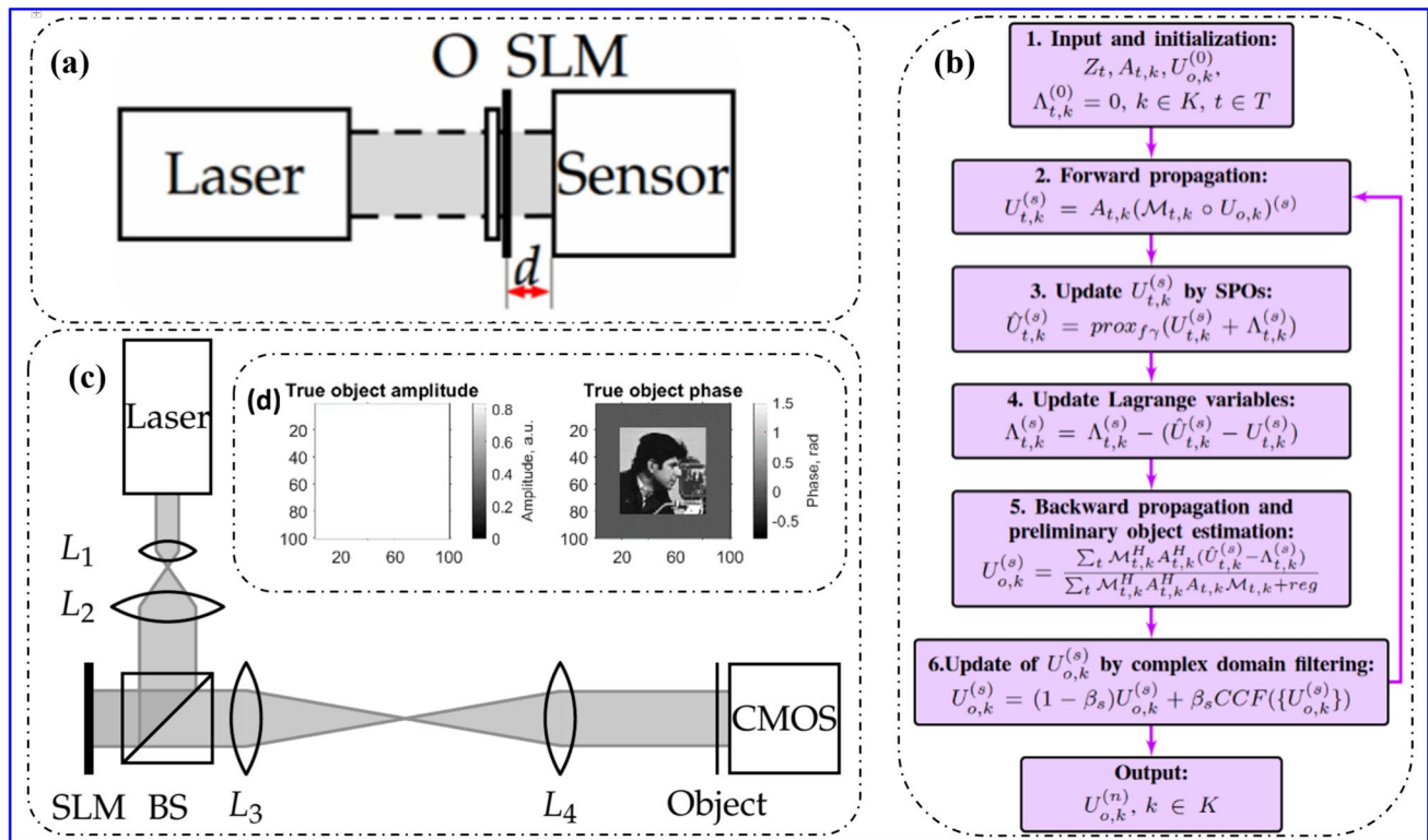
Fig. 30 a Schematic optical setup corresponding to our tests and data formation model; b HSPhR algorithm. c Reflective SLM-based experimental setup. The laser is a supercontinuum light source; L_1, L_2 are beam-expanding lenses; BS is a beamsplitter; ‘SLM’ is a Spatial
