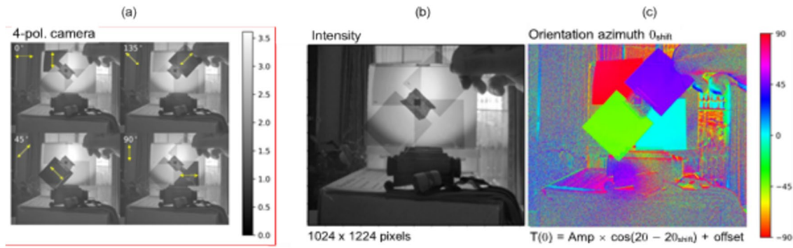
Fig. 53 a Four-polarisations (4-pol.) camera (CS505MUP1 Thorlabs) images of a room scene at wire-grid linear polarisers orientation \theta angles of 0, \pi/4 , \pi/2 , and 3\pi/4 (marked by arrows in top-left corners). Polarisers are on-chip integrated and the pixel size is 3.45 \mu\text{m} . The arrow markers on the dark linear polarisers (LPVISE2X2, Thorlabs) show a cross-Nikol condition since they polarise light perpendicular
